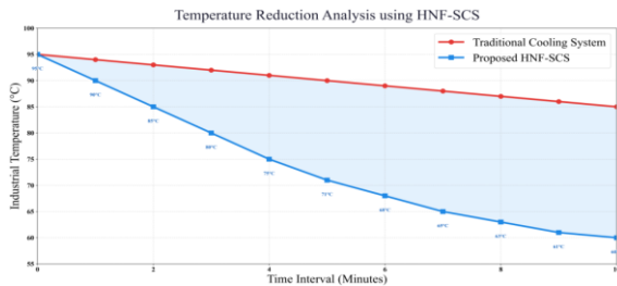
FIGURE 4: TEMPERATURE REDUCTION ANALYSIS USING HNF-SCS
