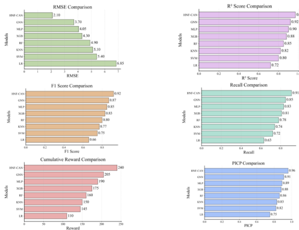
FIGURE 10: MODEL PERFORMANCE COMPARISON ACROSS MULTIPLE EVALUATION METRICS
