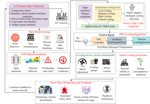
FIGURE 1: PROPOSED SMART COOLING SYSTEM WORKFLOW
